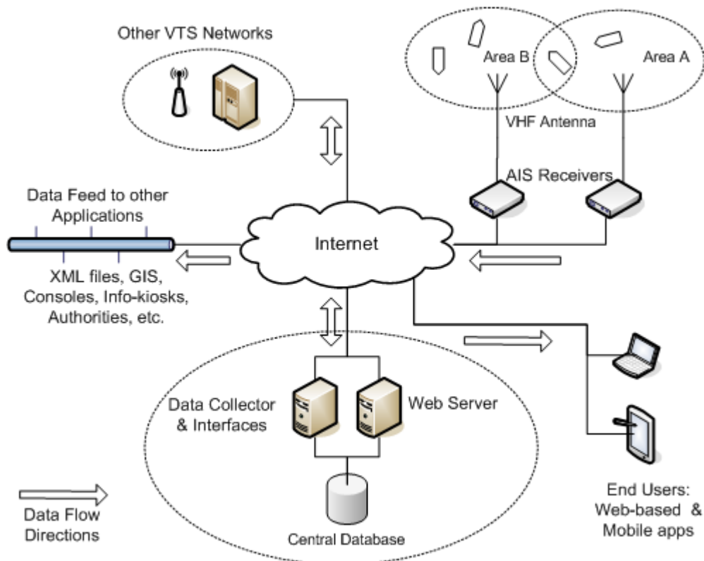
Figure 1: Generic Topology of VTMISS and peripheral equipment and applications
