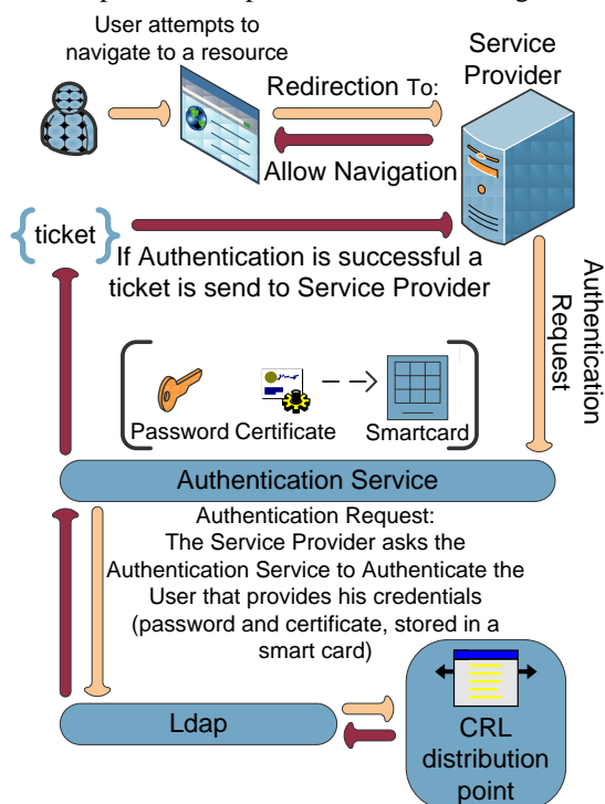
Figure 2: User Authorization
